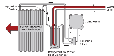
Heat Pump in Heating Mode
