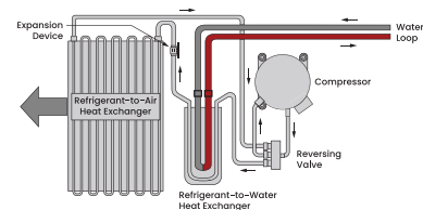
Heat Pump in Heating Mode
